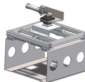
PLATE GRIPPER
