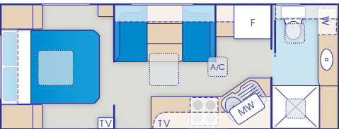
21' x 7'8"
